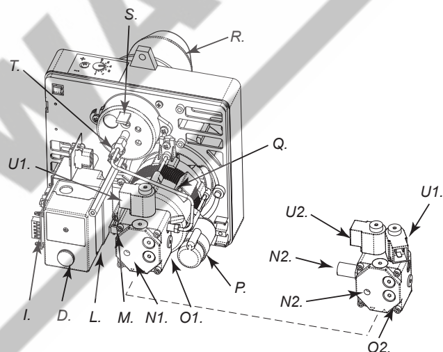
Figur 6 - Components burner
