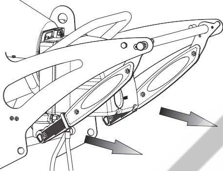
Figure 8 - Position close handles
