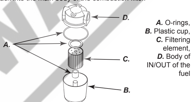
Figure 10 - Filter
