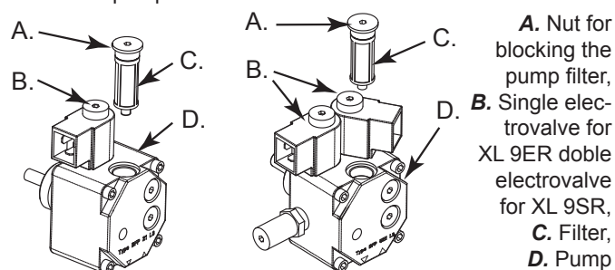
Figure 11 - Pomp of burner
