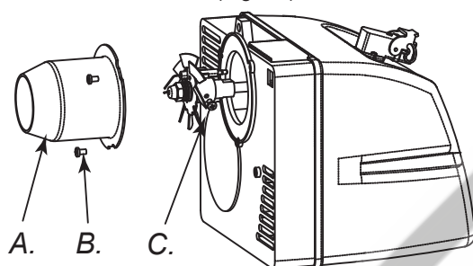
Figur 12 - Disassembly shell-burner
